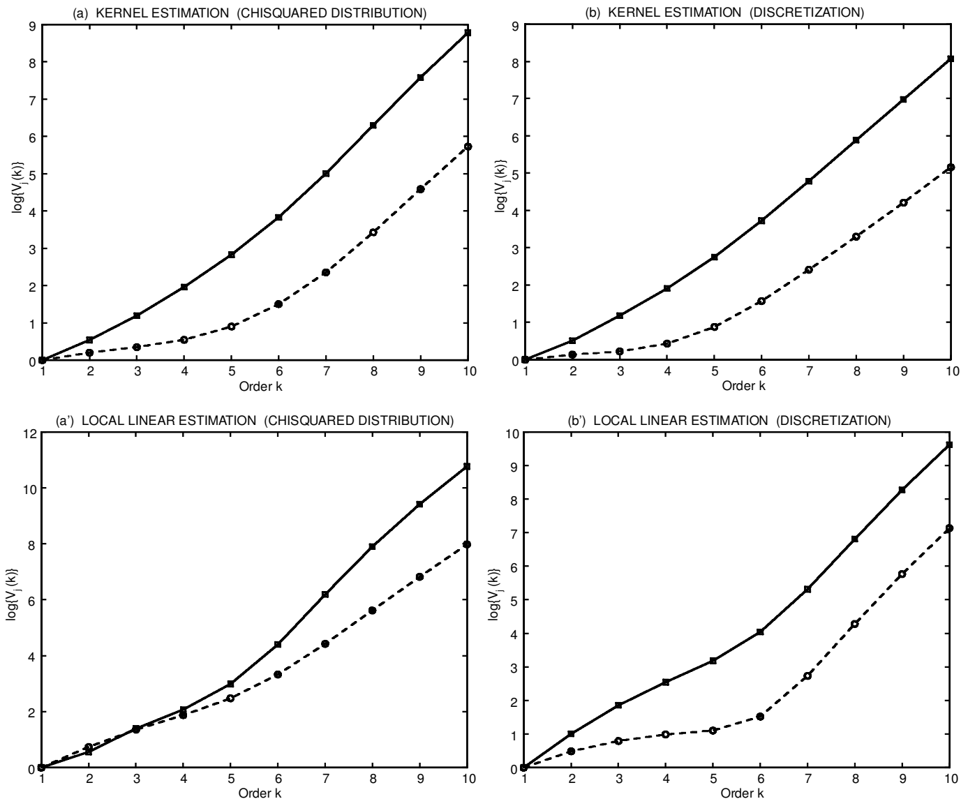
Figure 2. Simulated Values of \log\{V_j(k)\} Versus Order k for CIR Model dX_t = .21459(.08571 - X_t) dt + .07830X_t^{1/2} dW_t . The index j = 1 (---) refers to the drift estimator \hat{\mu}_{1,\Delta}(.1) ; j = 2 (—□) refers to the squared diffusion estimator \hat{\mu}_{2,\Delta}(.1) . Plots (a) and (a') are based on the same sets of sample paths generated by the noncentral chi-squared distribution, whereas plots (b) and (b') are based on the same sets of sample paths generated by the discretization scheme (31).
