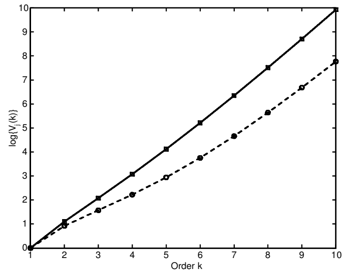
Figure 1. Theoretical Values of \log\{V_j(k)\} Versus Order k . The factors V_j(k) are given in Theorem 2, where j = 1 (—) refers to drift \mu(\cdot) and j = 2 (- -) refers to squared diffusion \sigma^2(\cdot) .
