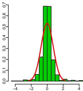
(b) Histogram
