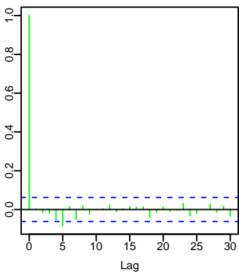
(e) ACF
