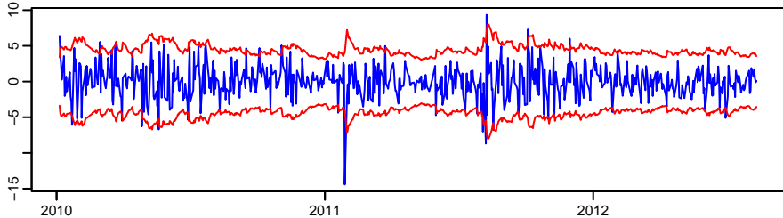
Daily returns of Ford stock
