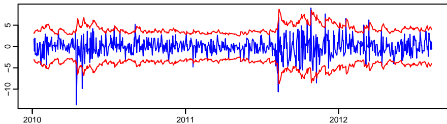
Daily returns of Goldman Sacks stock
