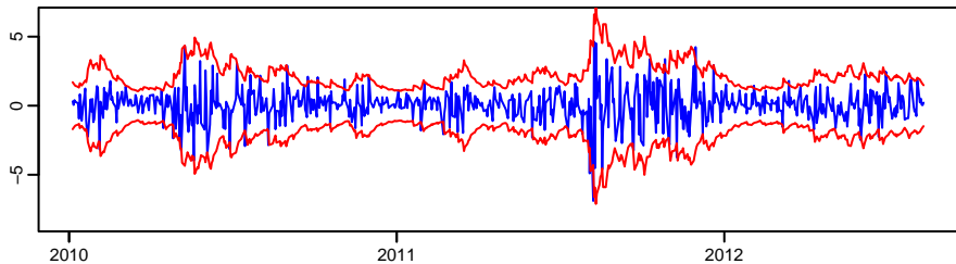
Daily returns of S&P500 index
