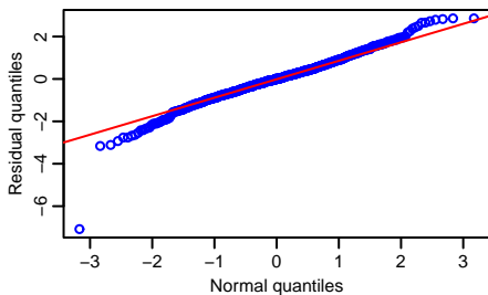
Ford, EGARCH(1,1)
