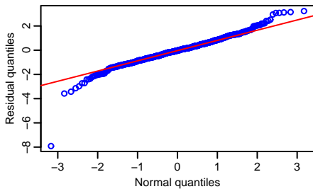
Ford, GARCH(1,1)
