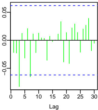
(c) ACF of residuals
