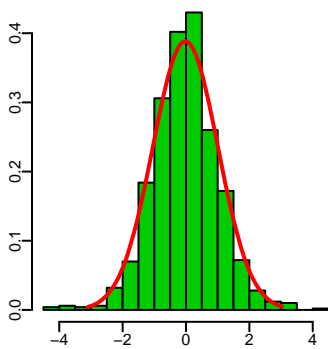
(b) Histogram
