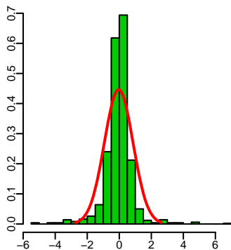
(b) Histogram
