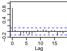
FTSE.M & FTSE.S
