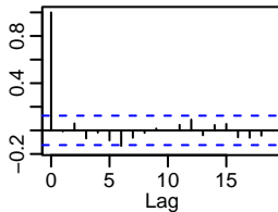
FTSE.SmallCap
