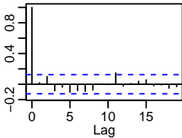
FTSE.S & FTSE.M
