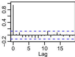
FTSE.MidCap
