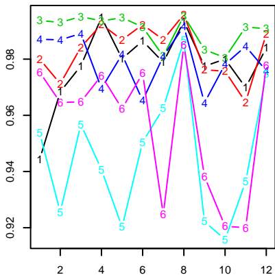
Multiple R-squares
