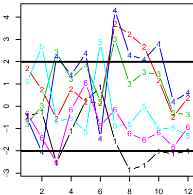
Estimated t-statistics
