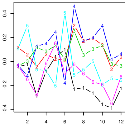
Estimated alphas
