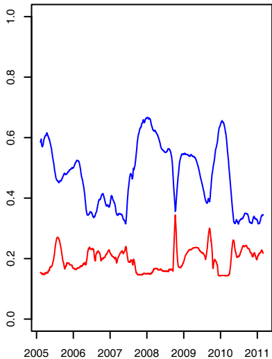
Variance explained ( w = 12 months)
