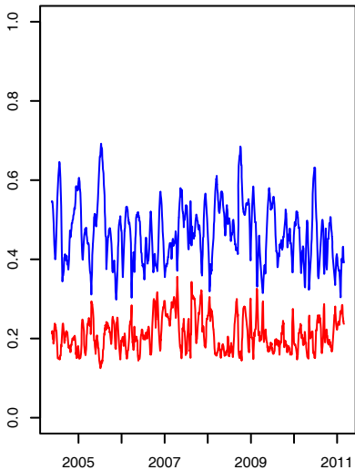
Variance explained ( w = 3 months)
