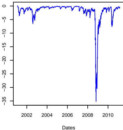
Covariance of SPX returns and VIX
