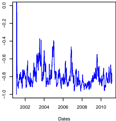
Correlation of SPX returns and VIX
