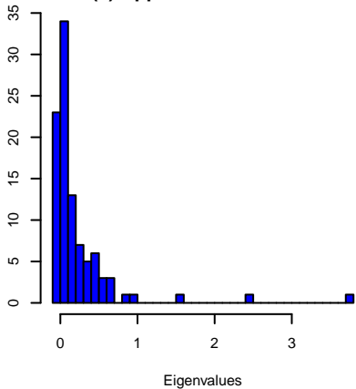
(c) Approx Factor Model
