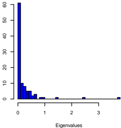
(c) Approx Factor Model
