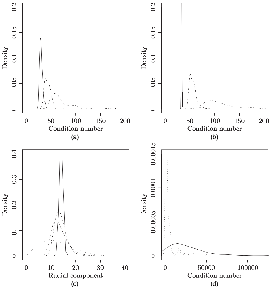
Fig. 10. (a), (b) Estimated densities of the condition number of \bar{p}^{-1}\bar{\mathbf{Z}}\bar{\mathbf{Z}}^T , based on 100 simulations, when \mathbf{Y} is Gaussian (—) and multivariate t with \nu = 20 (-----) and \nu = 10 (· · · · ·) degrees of freedom ((a) n = 100 , \bar{p} = 200 ; (b) n = 1000 , \bar{p} = 2000 ), (c) corresponding densities of the radial components of these spherically symmetric densities when \bar{p} = 200 , as well as the density of a scaled Weibull distribution with shape parameter 2 (· · · · ·), and (d) estimated condition number density of \bar{p}^{-1}\bar{\mathbf{Z}}\bar{\mathbf{Z}}^T in the Weibull case, with n = 100 , \bar{p} = 200 (· · · · ·) and n = 1000 , \bar{p} = 2000 (—)
