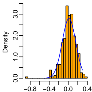
Monthly returns
