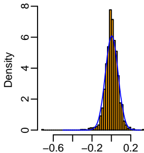
Weekly returns
