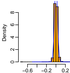
Daily returns
