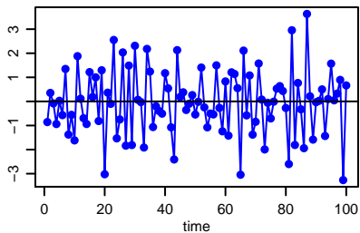
MA(2) process
