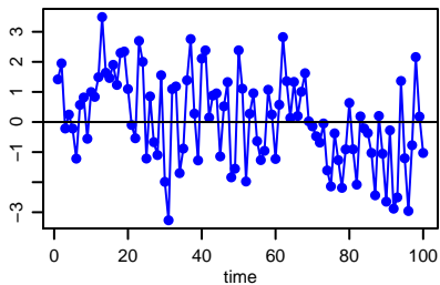
MA(4) process
