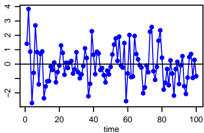
MA(4) process
