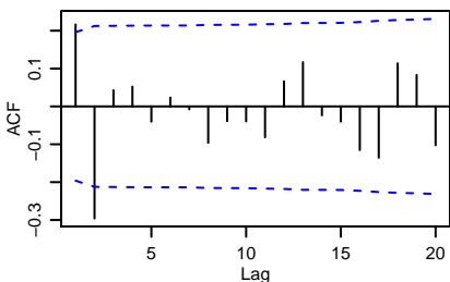
MA(4) process
