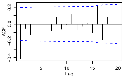
MA(2) process
