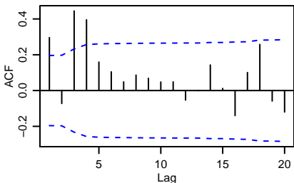
MA(4) process
