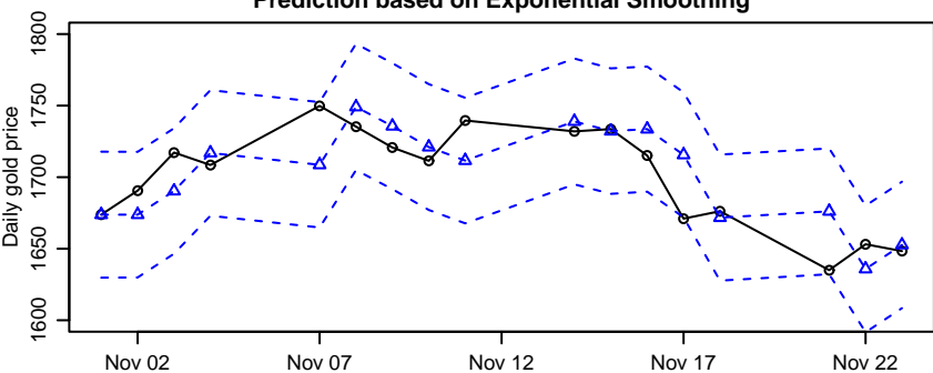
Prediction based on Exponential Smoothing
