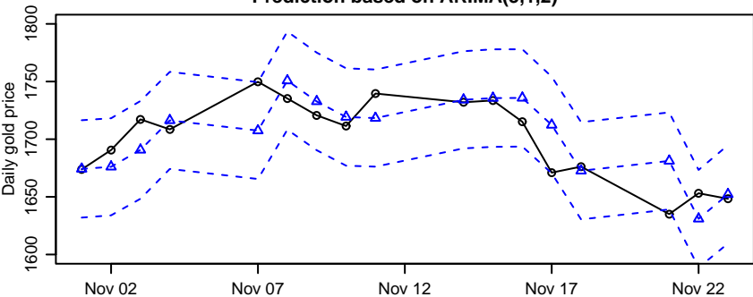
Prediction based on ARIMA(3,1,2)
