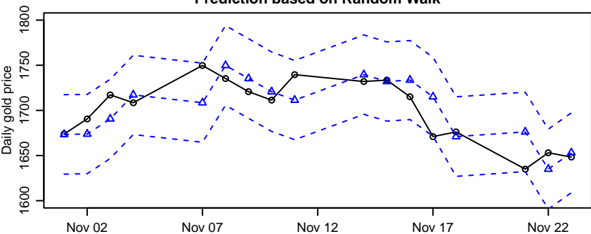
Prediction based on Random Walk
