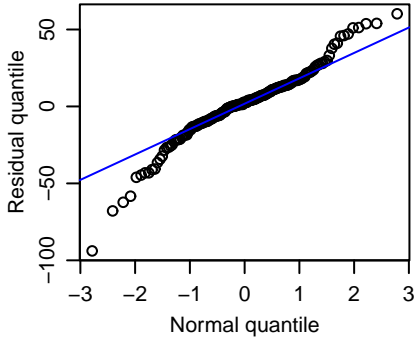
ARIMA(0,1,1)
