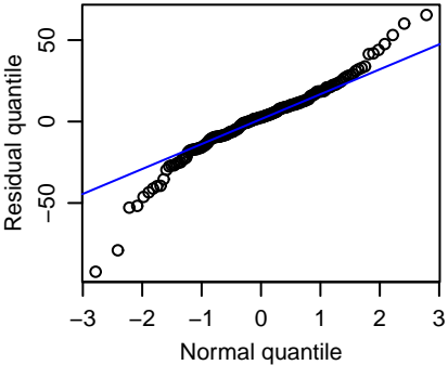
ARIMA(3,1,2)
