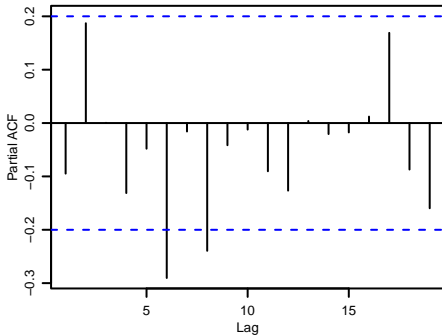
PACF of returns
